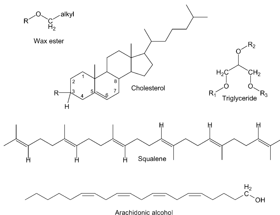
Fig. 1. Molecular structures of selected compounds discussed in the text. Displayed hydrogen atoms correspond to the protons measured in the NMR assay (see text). The labels R, R1, R2, and R3 represent any fatty acyl group.
