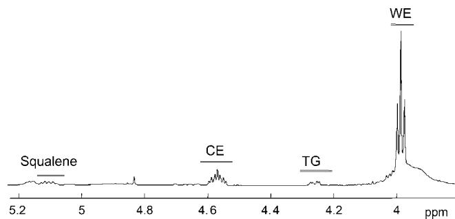
Fig. 7. Selected region of the 600 MHz proton NMR spectrum of a human meibum Sebutate ® extract.
