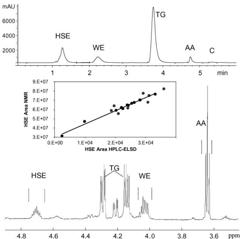
Fig. 2. Selected region of the 600 MHz proton NMR spectrum (bottom) and HPLC-evaporative light-scattering detection (ELSD; top) of a hamster ear punch extract. AA, arachidonic alcohol (internal standard); C, cholesterol; HSE, hamster sterol ester; TG, triglyceride; WE, wax ester. Inset shows a typical correlation between NMR and HPLC-ELSD results.
