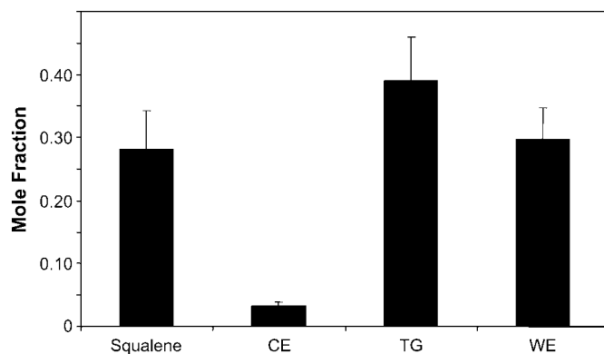
Fig. 5. Mole fractions of lipid components of a human Sebutate ® extract measured using the NMR method. Error bars indicate \pm SEM.
