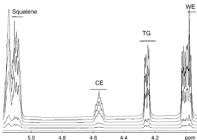
Fig. 4. Selected regions of the 600 MHz proton NMR spectra of the calibration standards. The concentrations of the components are (from bottom to top) 5, 50, 100, 500, 750, and 1,000 μM.
