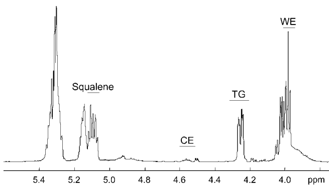
Fig. 3. Selected region of the 600 MHz proton NMR spectrum of a human Sebutape ® extract. CE, cholesteryl ester.
